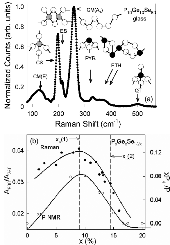
Figure 3. (a) Raman scattering of a ternary P_xGe_xSe_{1-2x} glass at x = 0.10 showing modes [15–21] of quasi-tetrahedral (QT) units ( 500\text{ cm}^{-1} ), ethylene-like (ETH) P_2Se_3 units ( 375\text{ cm}^{-1} ), pyramidal (PYR) P(Se_{1/2})_3 units ( 330\text{ cm}^{-1} ), Se_n chain mode (CM) at 250 and 140\text{ cm}^{-1} , corner-sharing (CS) and edge-sharing ES Ge(Se_{1/2})_4 units near 200 and 217\text{ cm}^{-1} respectively [17]. (b) Shows a plot of the Raman scattering strength of the QT mode normalized to the CM at 250\text{ cm}^{-1} in open circles, while the filled circles give concentrations of the QT units inferred from ^{31}\text{P} NMR, [21].
